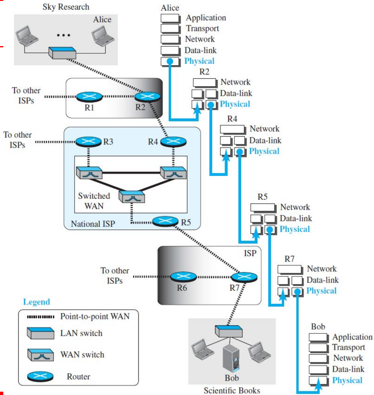
Figure 3.1 Communication at the physical layer
